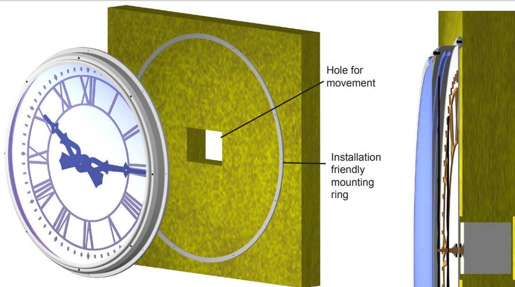
Model 400 Flush Mount No Tub - Non-Illuminated
