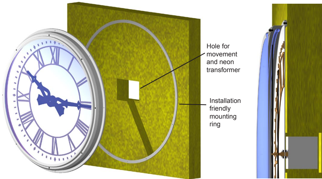
Model 400 Flush Mount No Tub - Front Illuminated
